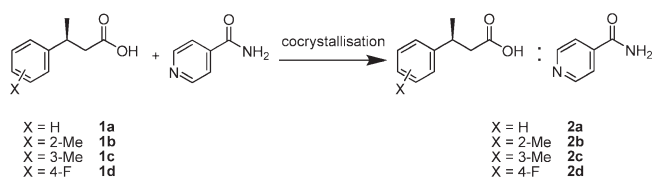
FIGURE 2. Co-crystallization of the 3-arylbutanoic acids with isonicotinamide.
