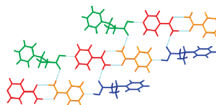
FIGURE 3. Hydrogen bonding interactions in ( S )- 2a . The different colors indicate unique, symmetry-independent ( S )- 2a (green and blue) and isonicotinamide (red and orange) molecules. The same motif is formed in ( S )- 2c , ( S )- 2d , ( \pm )- 2b , and ( \pm )- 2c , see the Supporting Information.
