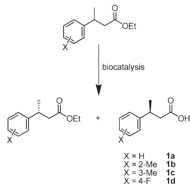
FIGURE 1. The enzymatic biotransformation employed in this work. 5
