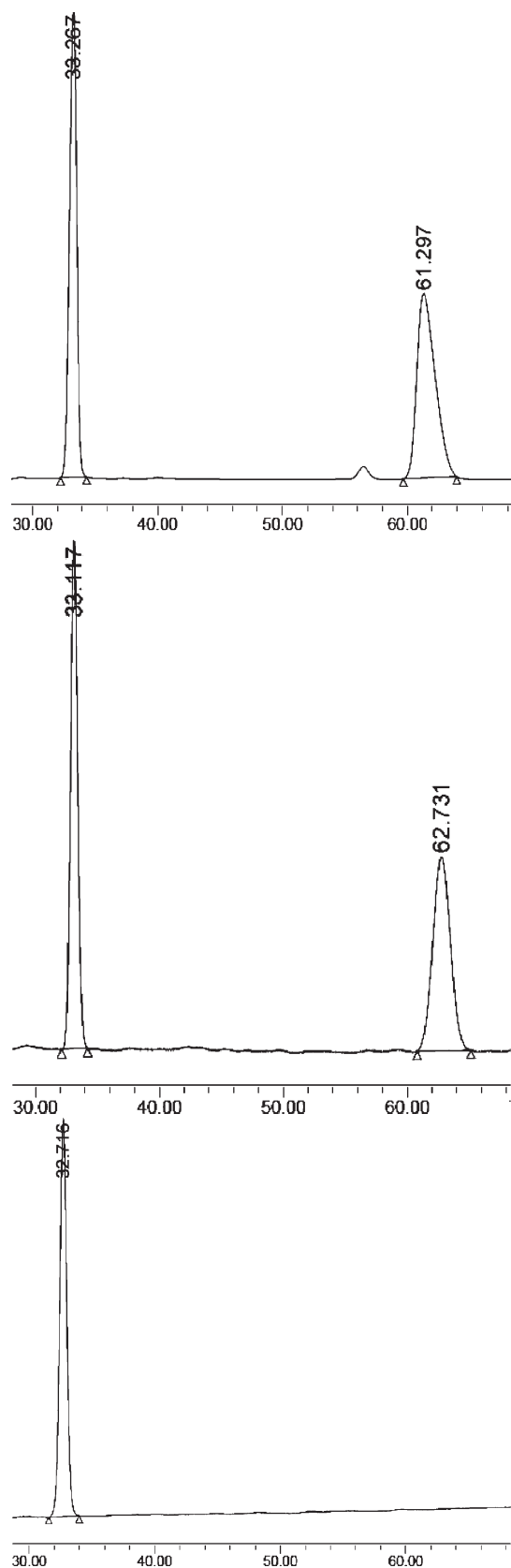
FIGURE 5. Chiral HPLC trace for (±)-1b, top; (±)-2b, middle; and (S)-2b, bottom. For (±)-2b and (S)-2b, the data are obtained by using the individual crystal from the single crystal analysis.
